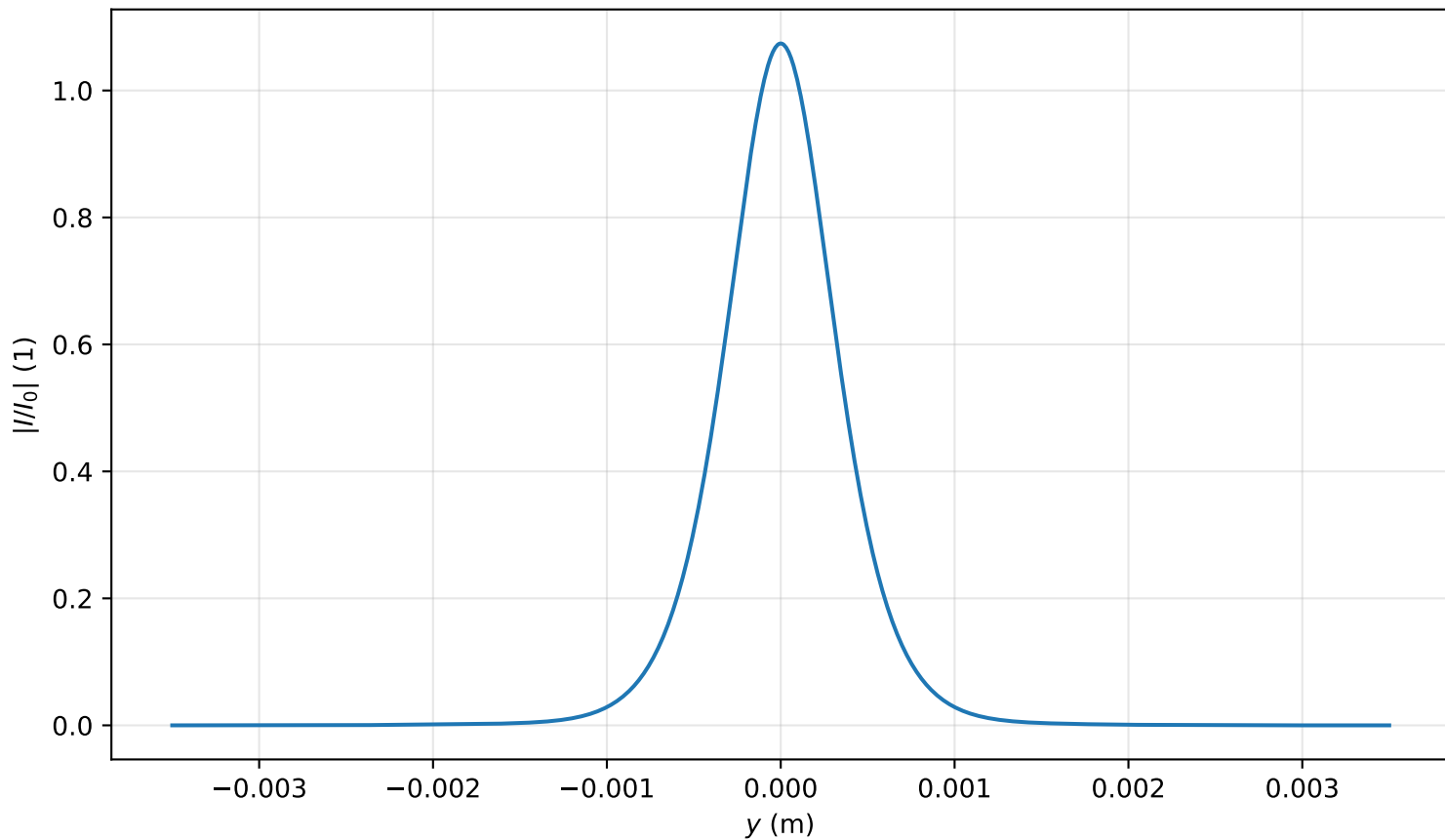
Intensity profile I(x=0, y, z=3.105)/I_0 , P_{in}=0.8P_{cr} , artificial time
